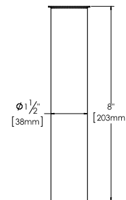
Flanged Tailpiece Attaches to 314DC Series Cable-Driven Bath Wastes and Integral Bath Wastes.
